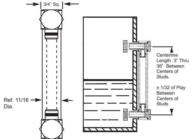
Mounting Bolts with Adapters
